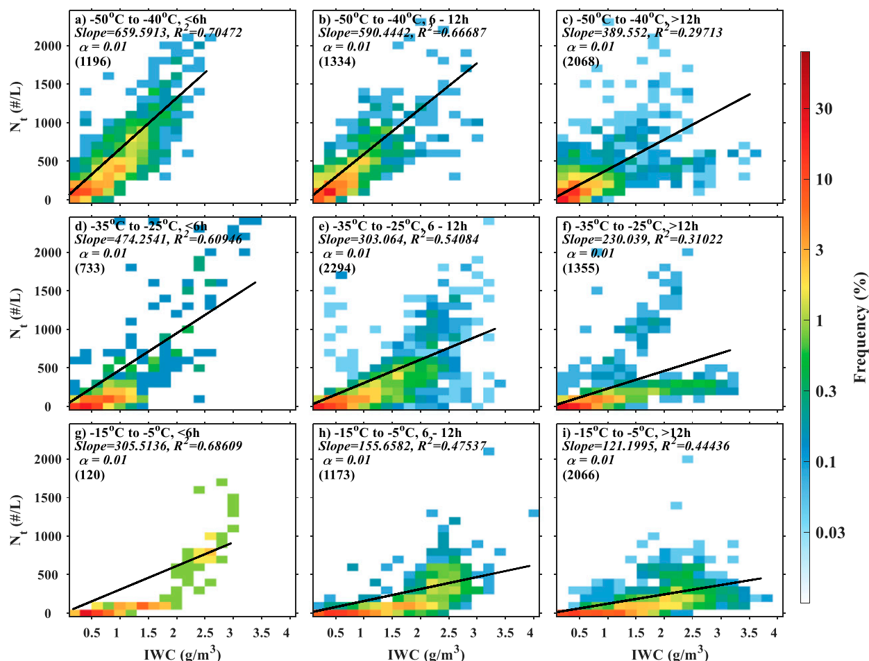
FIG. 14. As in Fig. 5, but for MCSs sorted by age ( <6 , 6–12, and >12 h) rather than for updrafts, downdrafts, and stratiform regions.
