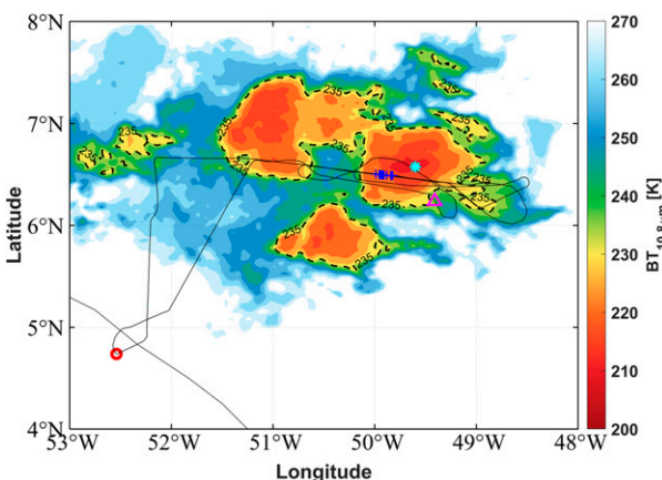
FIG. 1. GOES-13 measured brightness temperature ( BT_{10.8\mu m} ) at 1115:00 UTC 15 May 2015 with flight track of Falcon 20 overlaid with black line for flight 13. The black dashed line shows the temperature contour line at 235 K. Red circle indicates location of Cayenne (4.74°N, 52.5°W), blue points indicate where IKP2 IWC > 1.5 \text{ g m}^{-3} and MMD < 400 \mu m between -50^\circ \leq T \leq -40^\circ \text{C} , magenta triangle and cyan asterisk ( BT_{10.8\mu m} = 213.6 \text{ K} ) denote location of aircraft and of MCS convective core at 1115:00 UTC, respectively.
