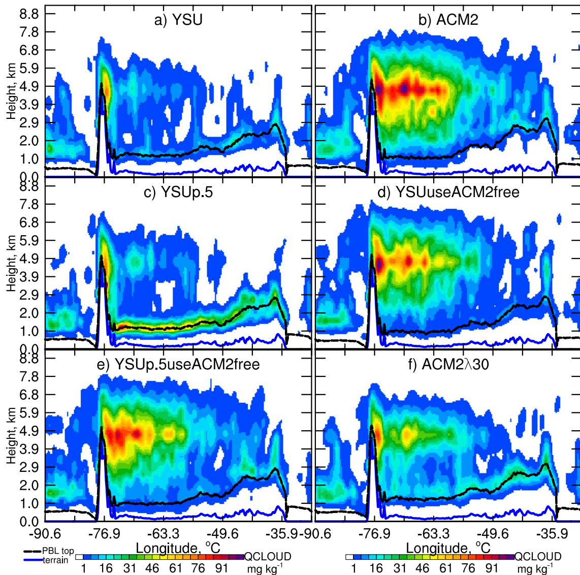
Figure 7. Cross-section of cloud water over the Amazon in January–February 2019 simulated by (a) YSU and (b) ACM2, (c) YSU p.5, (d) YSUuseACM2free, (e) YSU p.5useACM2free, (f) ACM2 \lambda 30 at 17 UTC. The location of these cross-sections is marked in Figure 5j.
