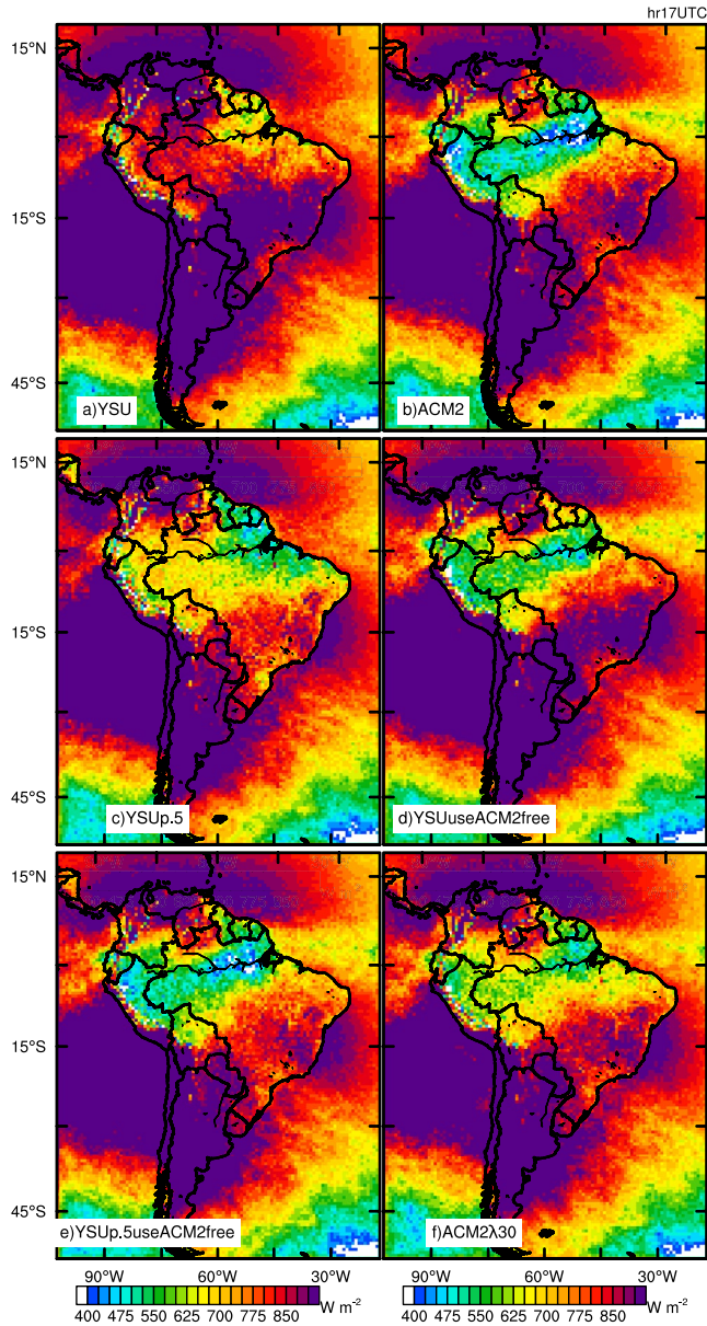
Figure 8. Average surface downward shortwave radiation at 17 UTC during January–February 2019 simulated by (a) YSU, (b) ACM2 and four sensitivity simulations (c) YSU p.5 , (d) YSUuseACM2free, (e) YSU p.5 useACM2free, (f) ACM2 \lambda 30.
