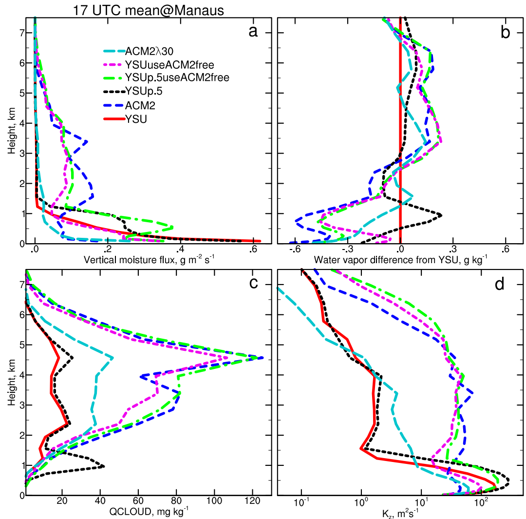
Figure 10. Mean profiles of (a) vertical moisture flux, (b) water vapor difference from that simulated by YSU, (c) cloud water mixing ratio ( Q_{CLOUD} ), and (d) vertical mixing coefficient ( K_z ) at 17 UTC during January–February 2019 at Manaus (location marked in Figure 9b) simulated by YSU, ACM2 and four sensitivity simulations YSU p.5 , YSU useACM2free , YSU p.5useACM2free , ACM2 λ30 .
