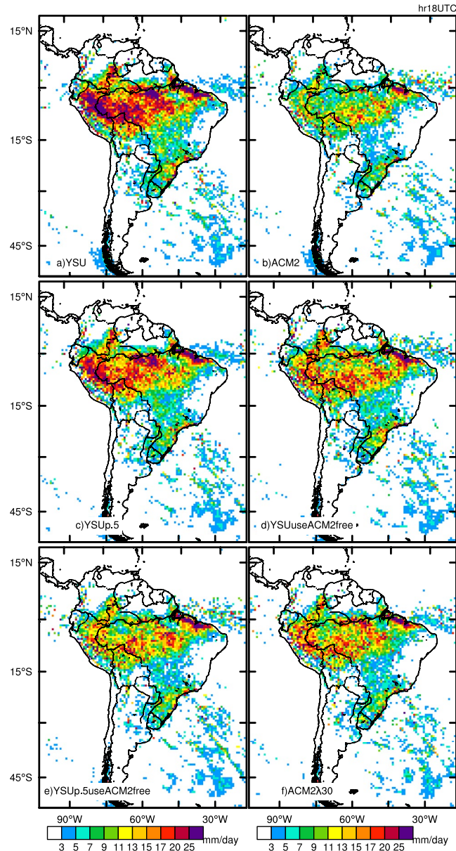
Figure 11. Average precipitation rate at 18 UTC during January–February 2019 simulated by (a) YSU, (b) ACM2 and four sensitivity simulations (c) YSU p.5 , (d) YSU useACM2free , (e) YSU p.5useACM2free , (f) ACM2 λ30 .
