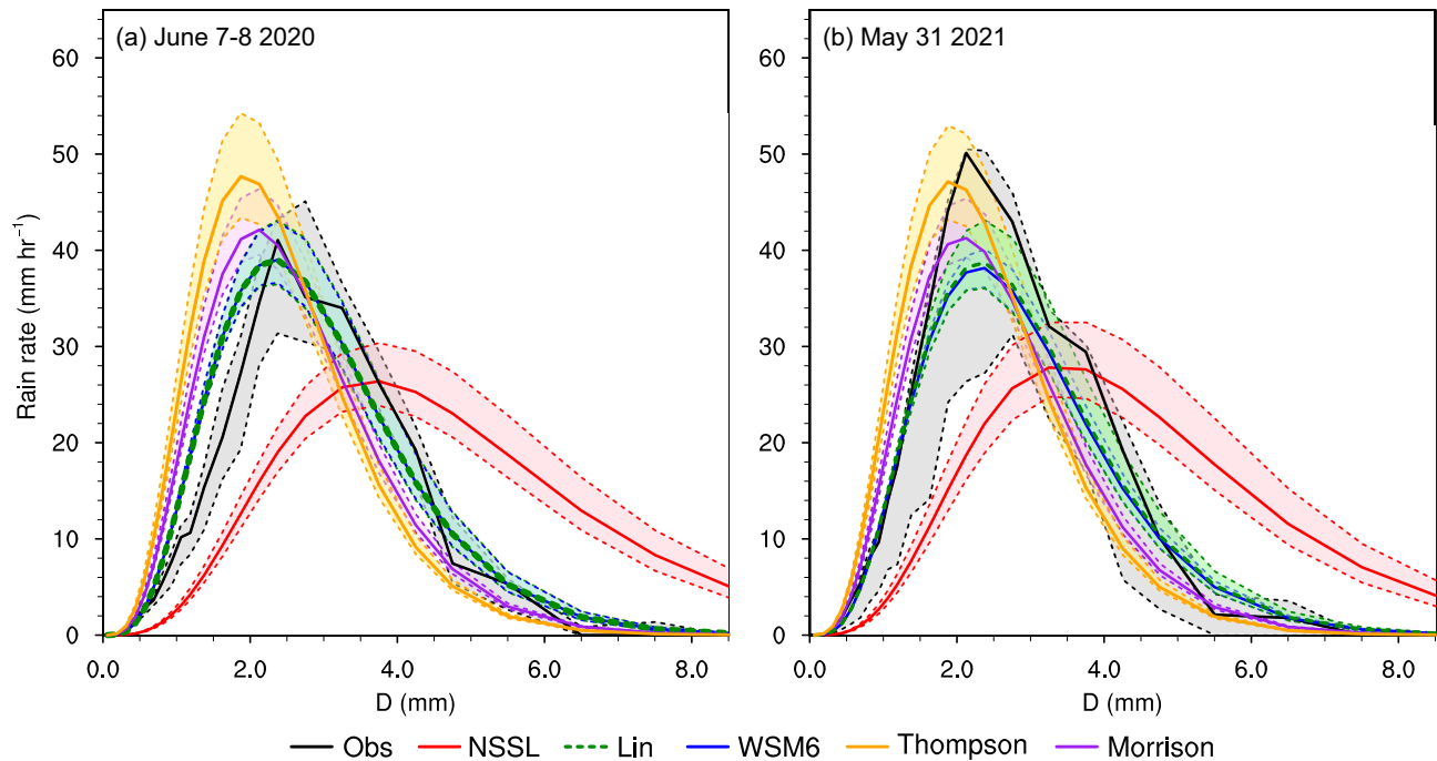
FIGURE 18 As in Figure 3, but for observed and simulated distribution of rain rate for the cases (a) during June 7–8, 2020, and (b) on May 31, 2021. Only the distribution data with integral precipitation intensity R \geq 100 \text{ mm} \cdot \text{hr}^{-1} are shown.
