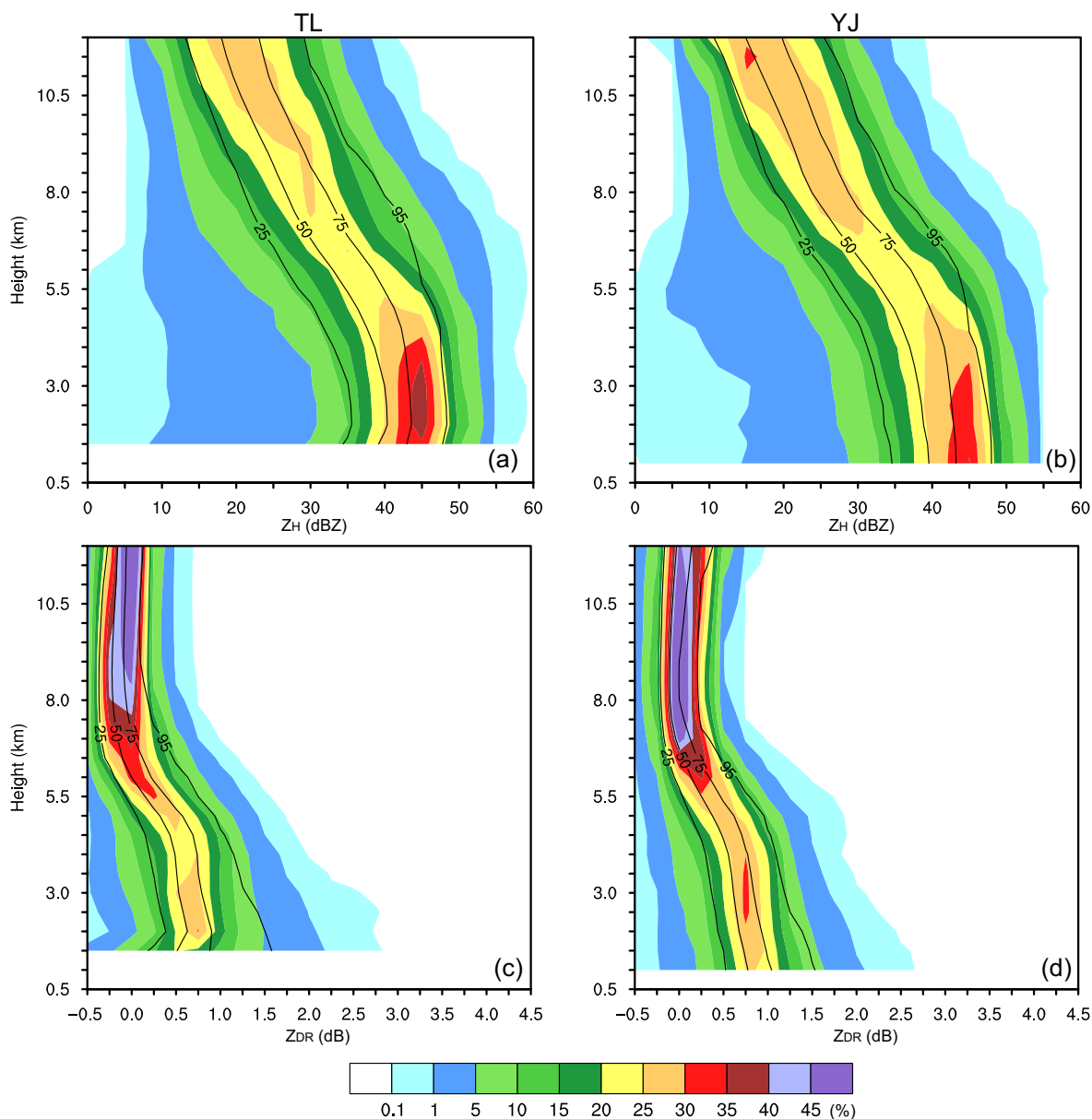
FIGURE 4 The contoured frequency by altitude diagrams (CFADs, shaded) of the observed (a, b) reflectivity ( Z_H ) and (c, d) differential reflectivity ( Z_{DR} ), and the corresponding cumulative CFADs (black contours) over the key areas TL (left) and YJ (right) during the maximum hourly rainfall period. Black contours indicate the cumulative frequencies of 25%, 50%, 75%, and 95% respectively. [Colour figure can be viewed at wileyonlinelibrary.com ]
